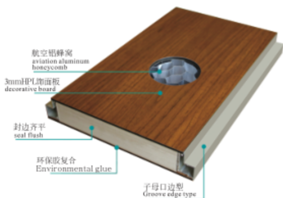
FA-10 HPL复合板结构图 FA-10 composite plate structure
