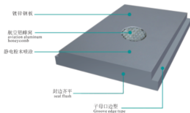
FA-10 VCM复合板结构图 FA-10 composite plate structure
